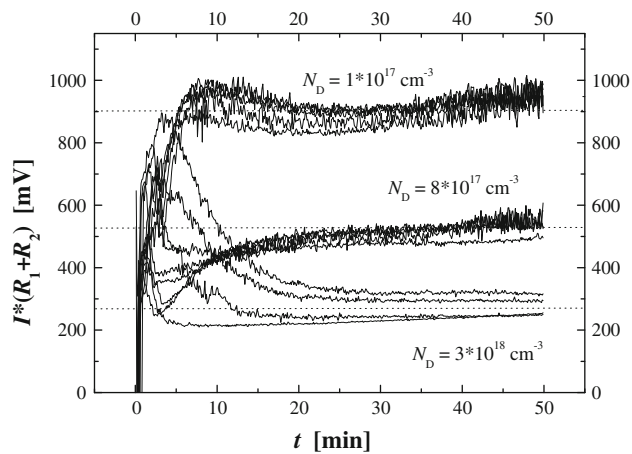
Fig. 3 Potential drop U_{SCR} = I(R_1 + R_2) over the space-charge-region (SCR). Several lines correspond to different etching potentials in the aforementioned respective etching potential windows. The curves are constant after an initial nucleation phase and dependent on N_D
