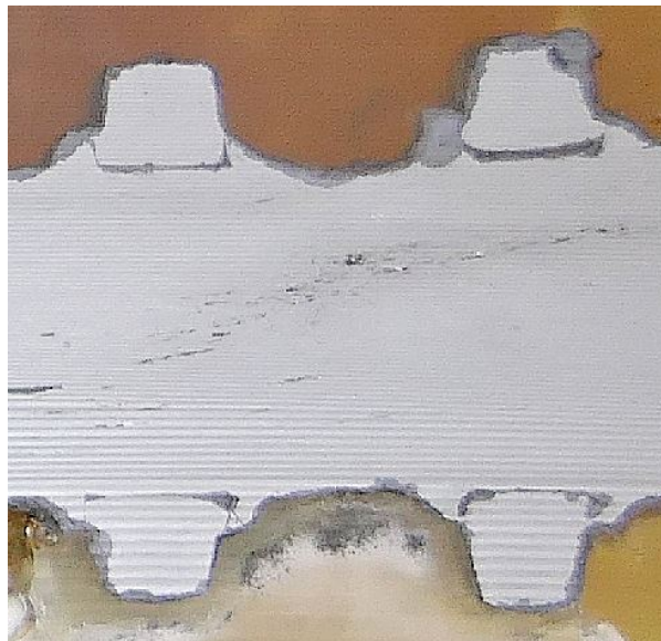
Cut showing the crimping around the rings
